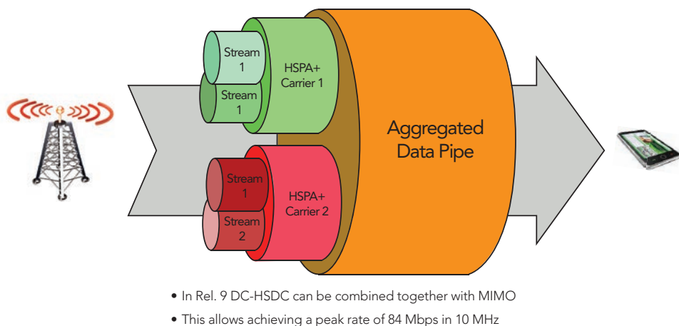
Figure 3 : Rel-9 - graphical representation of MIMO combined with CA
