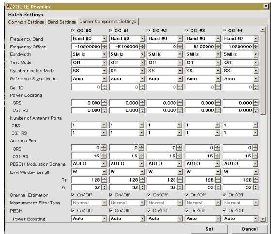
Figure 30 : Carrier setting - measurement software MX269020A-001
