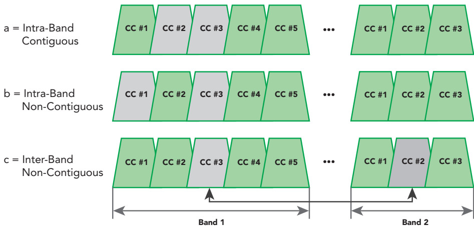
Figure 10 : Different type of CA allocation in LTE-A
