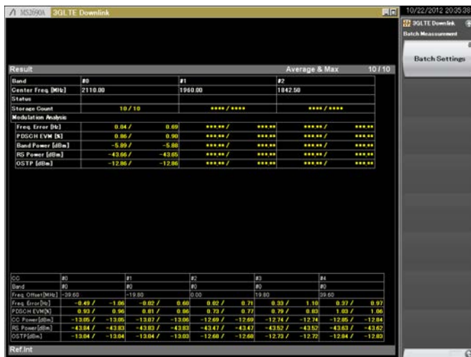
Figure 28 : Measurement software MX269020A-001- Example of Batch Measurement Result Display (Component Carrier: CC #0 to #4)
