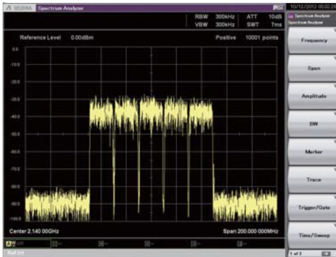
Figure 27 : Spectrum analyzer MS269xA/MS2830A - Example of Spectrum of LTE-Advanced signal (Component Carrier: Bandwidth 20 MHz, 5CC)
